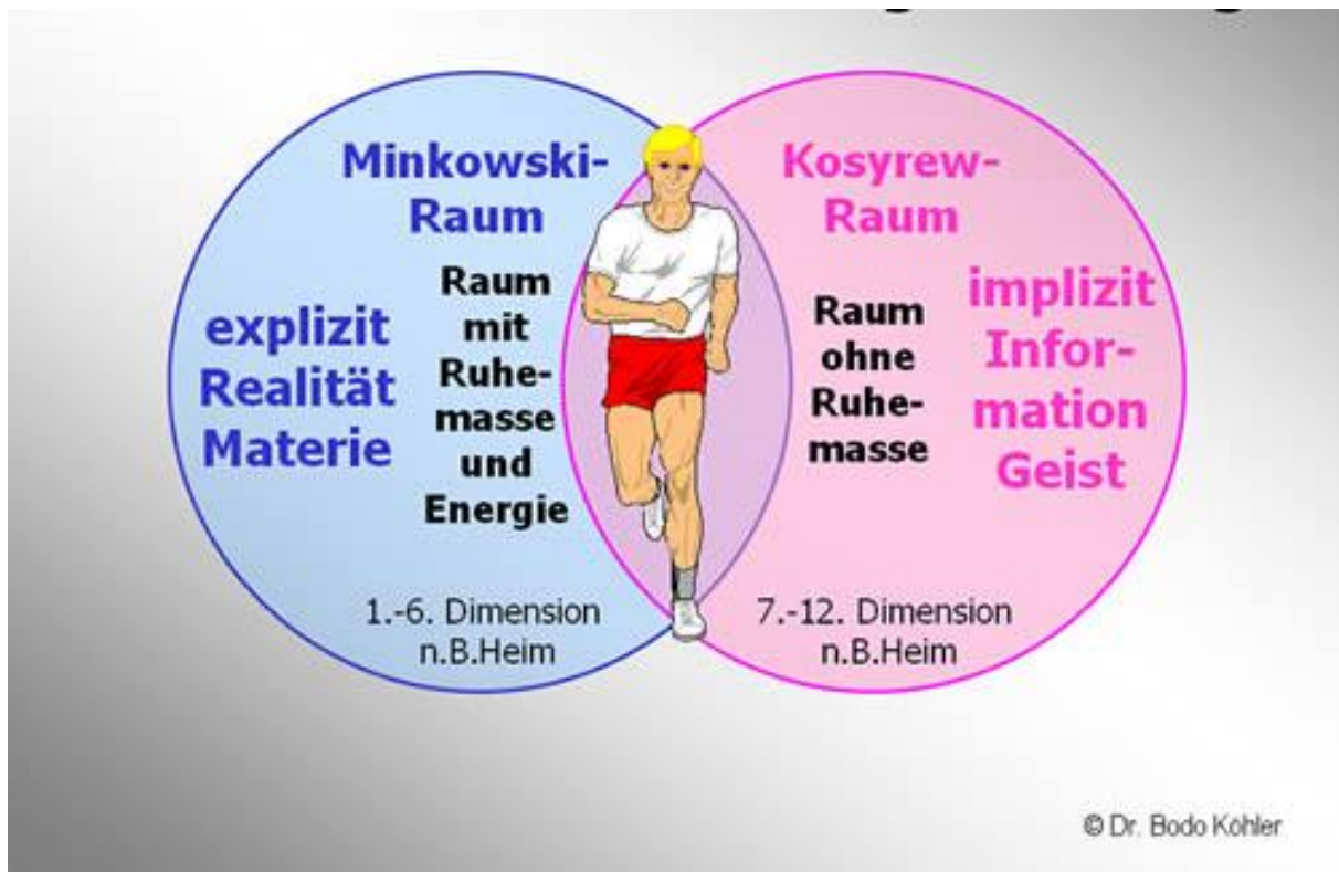
Figure. Dimensions according to B. Heim
