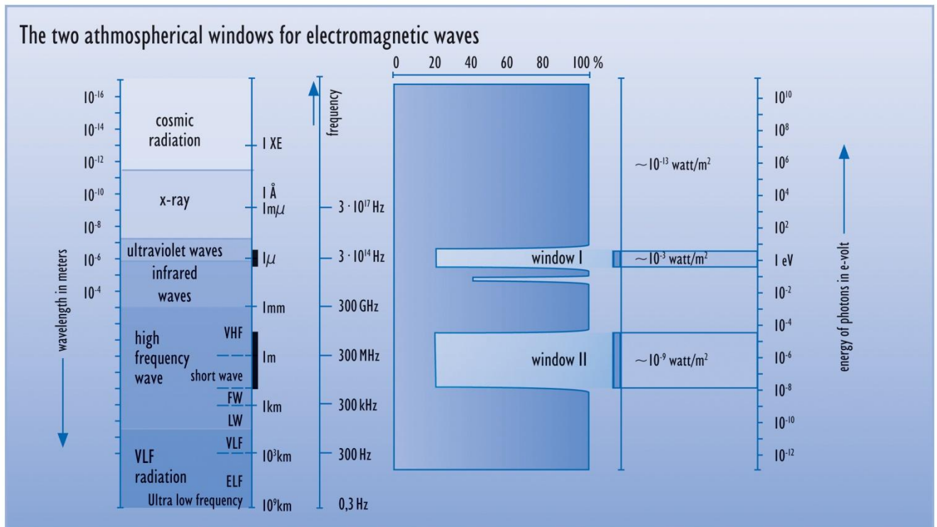
Figure: The two “atmospheric windows” for electromagnetic radiation.
