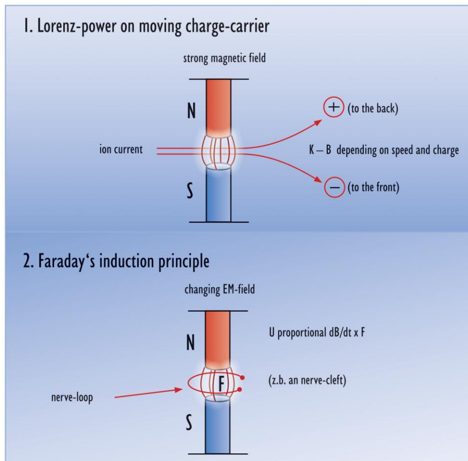
Figure: LORENTZ force on moving charge carriers and Faraday's law of induction
