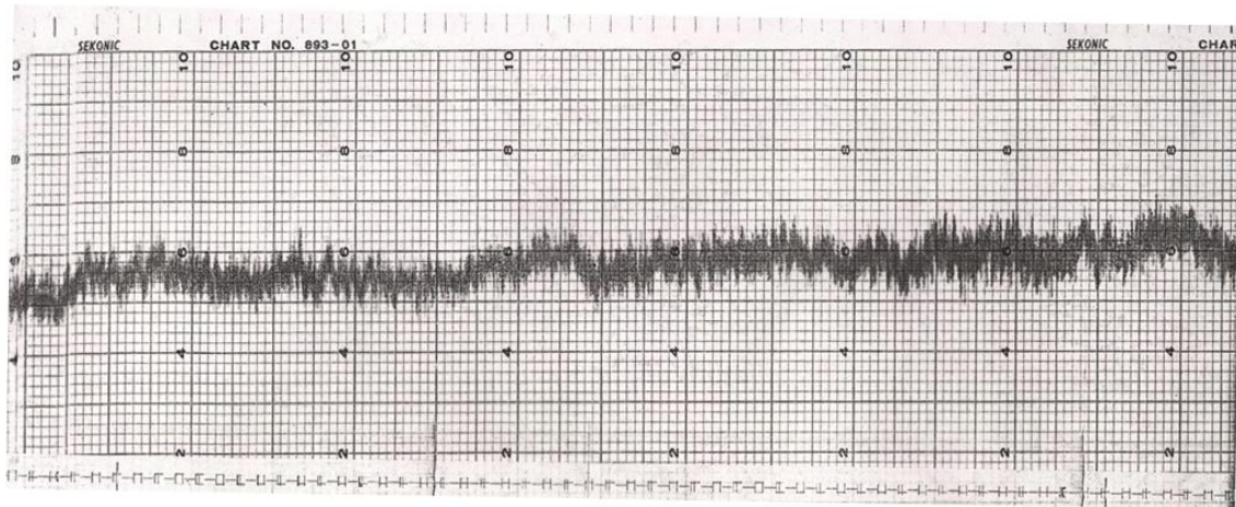
Figure: Rhythmic fluctuations of the Earth's magnetic field
