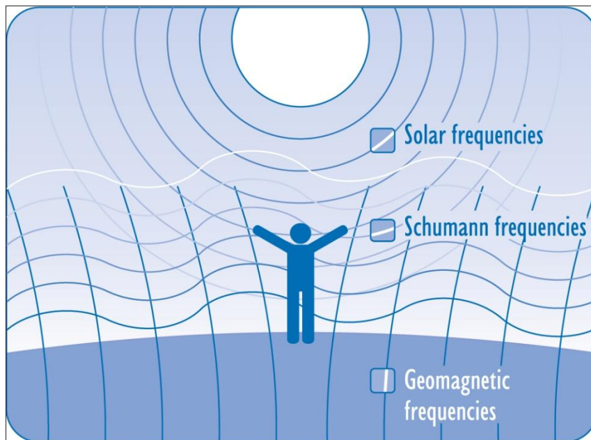
Figure: The three Biological Normals: Schumann-, geomagnetic- and solar-frequency spectra
